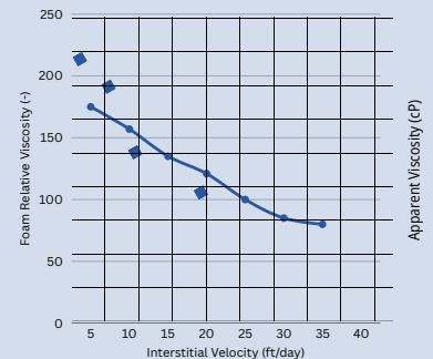
Interstitial Velocity (ft/day) Steam Foam viscosity measured in coreflood experiment at 220°C in native core and in the presence of 12% residual oil saturation.
